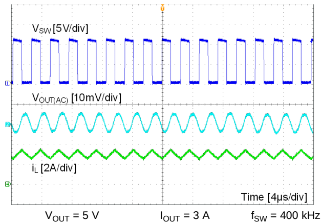
Figure 24. CCM Mode
