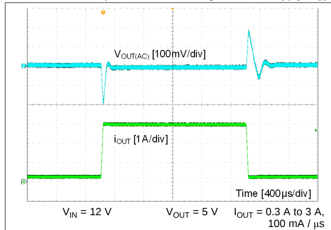
Figure 30. Load Transient
