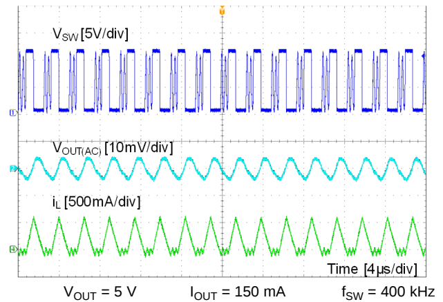
Figure 25. DCM Mode
