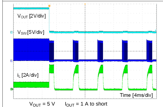
Figure 32. Short Protection
