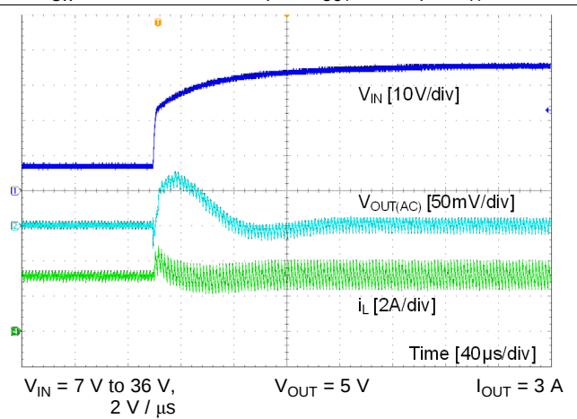
Figure 31. Line Transient
