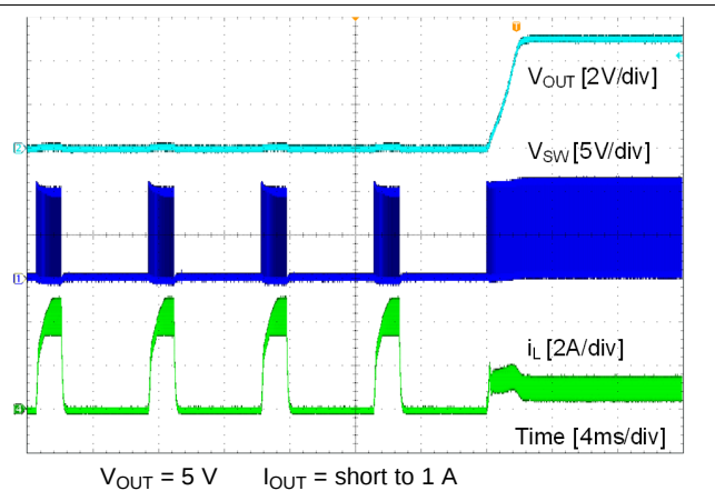
Figure 33. Short Recovery
